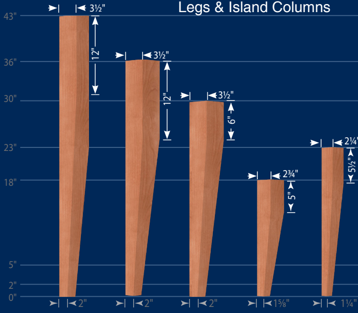
Bar Leg 121052-350 Island Leg 101052-350 Table Leg 91052-350 Coffee Table Leg 81052-275 End Table Leg 71052-225
