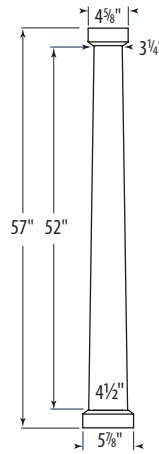
Bar Leg 121054-350 Island Leg 101054-350 Table Leg 91054-350 Coffee Table Leg 81054-275 End Table Leg 71054-225
