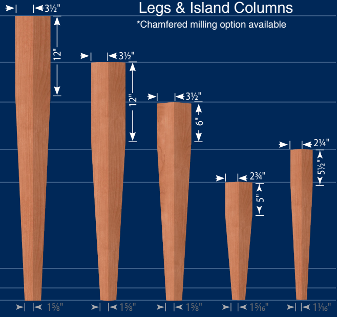
Bar Leg 121054-350 Island Leg 101054-350 Table Leg 91054-350 Coffee Table Leg 81054-275 End Table Leg 71054-225
