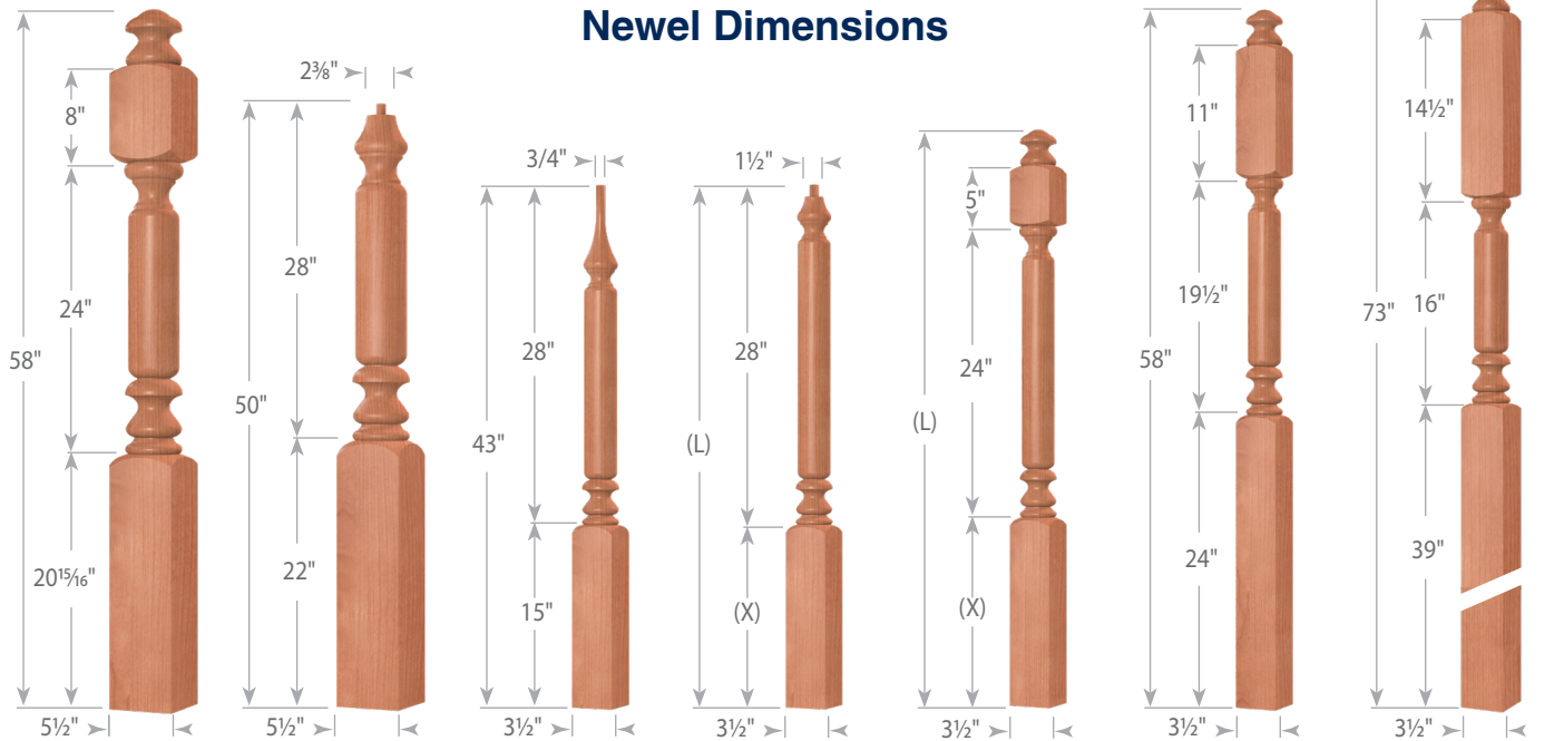
Post to Post Estate Newel 4750-550
