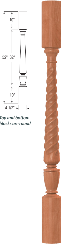
Fireplace Column Example
