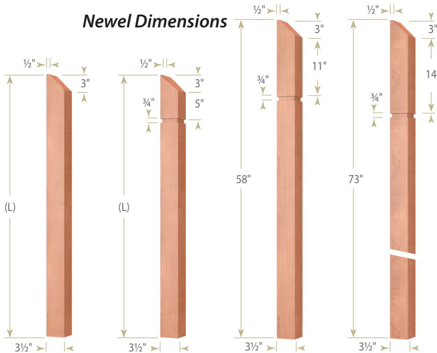
Post to Post Newel
