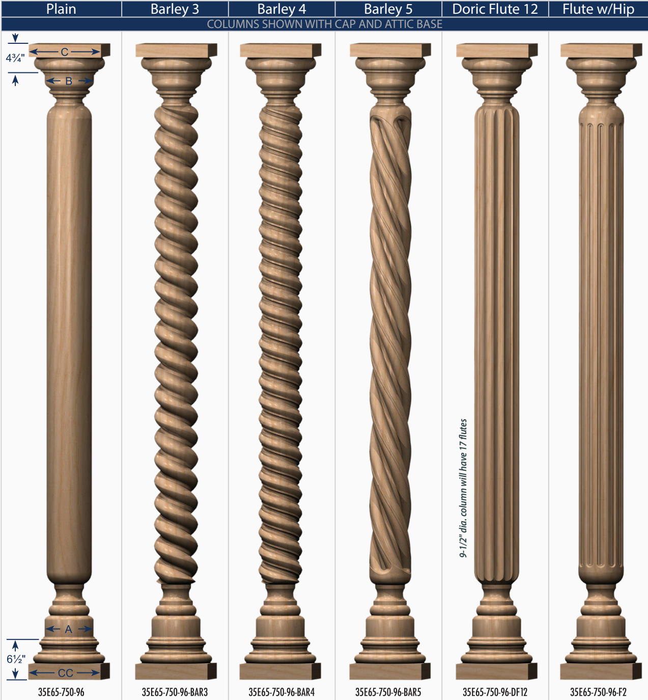
DECORATIVE SOLID ROUND COLUMN DIMENSIONS
