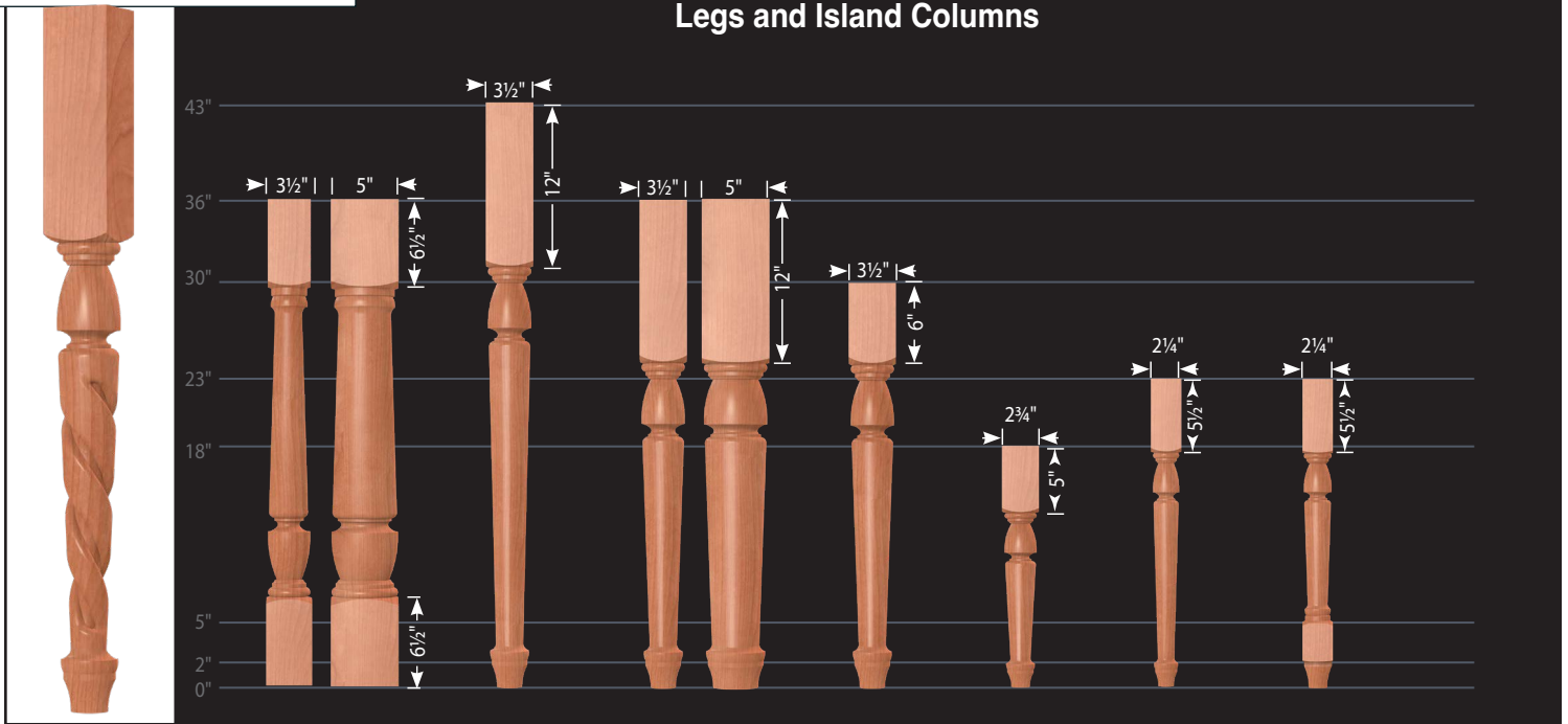
Island Leg Example 102005-350-BAR2 Island Column 12005-350 12005-500 Bar Leg (Footed) 122005-350 Island Leg (Footed) 102005-350 102005-500 Table Leg (Footed) 92005-350 Coffee Table Leg (Footed) 82005-275 End Table Leg (Footed) 72005-225 End Table Leg (w/stretcher block) 62005-225
