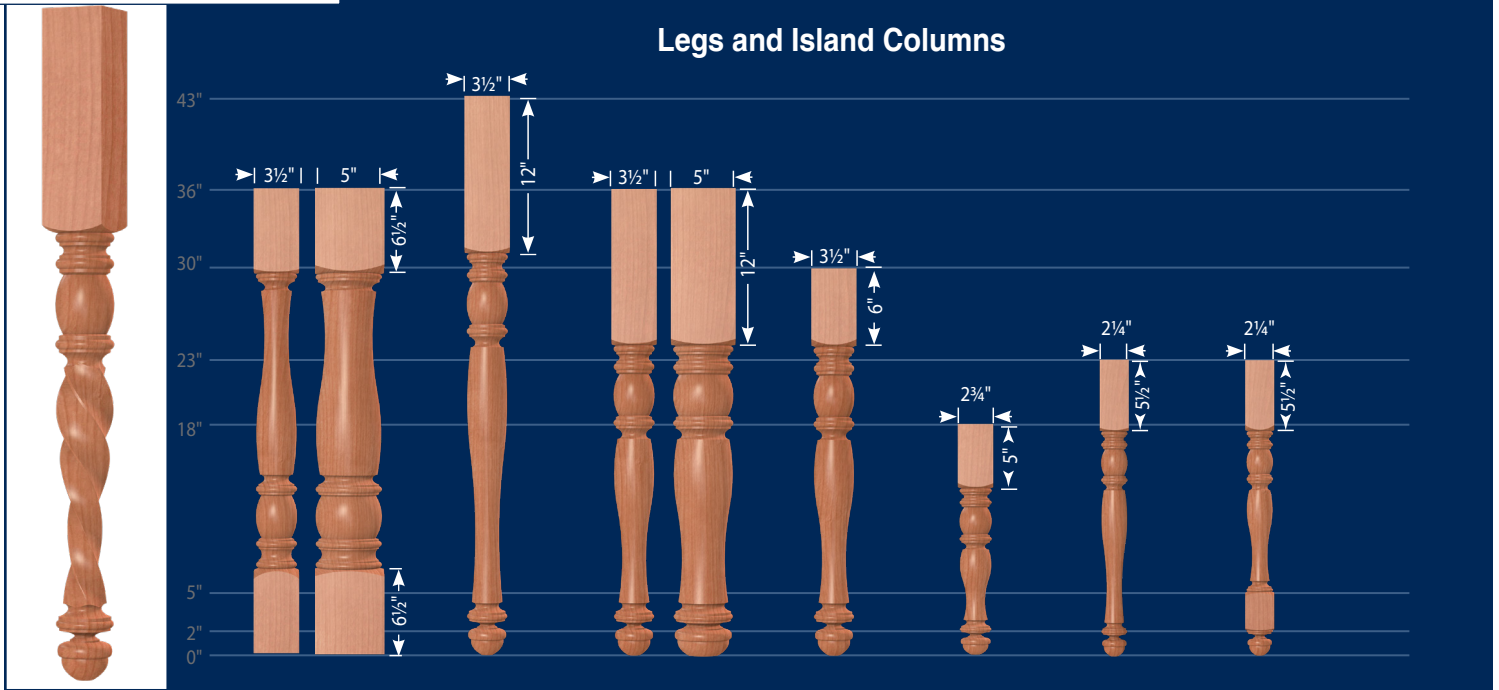
Island Leg Example 12105-350-RIB2 Island Column 12105-350 12105-500 Bar Leg (Footed) 122105-350 Island Leg (Footed) 102105-350 102105-500 Table Leg (Footed) 92105-350 Coffee Table Leg (Footed) 82105-275 End Table Leg (Footed) 72105-225 End Table Leg (w/stretcher block) 62105-225
