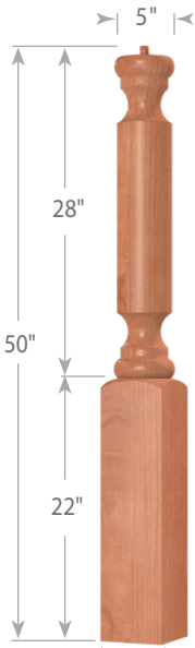
Pin Top Estate Newel 3616-550
