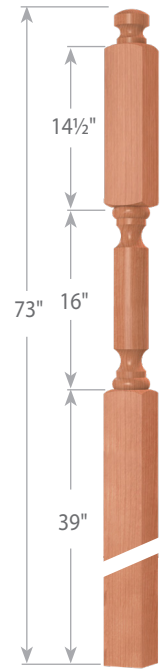
Intermediate Landing Newel 3646-350
