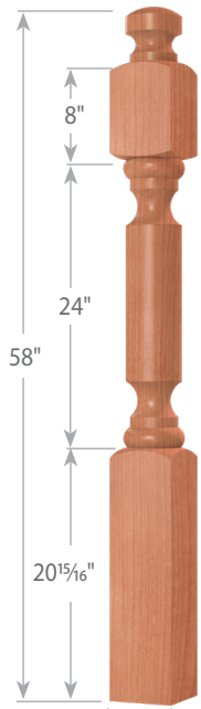
Post to Post Estate Newel 3650-550
